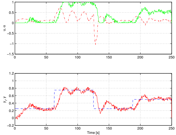
Fig. 3. Simulation of the controlled system. Top: scheduling variable \alpha (green full line) and control signal u (red dash-dot line). Bottom: reference signal y_r (blue dash-dot line) and controlled output y (red full line).
