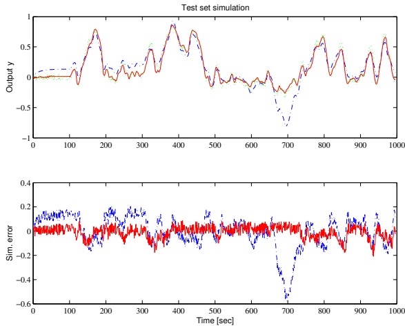
Fig. 2. Top: open-loop simulation of the test set (green dotted line) by the linear (blue dash-dot line) and the MLP model (red full line). Bottom: open-loop simulation errors for the linear (blue dash-dot line) and the MLP model (red full line).
