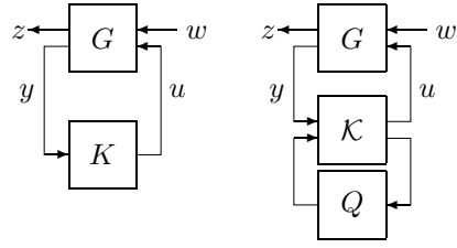
Fig. 1. The interconnection of the system G and the controller K (left). The controller is parameterized by means of a star product between an augmented system \mathcal{K} and a stable parameter system Q (right).
